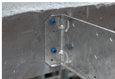
Titen® 2 screw
