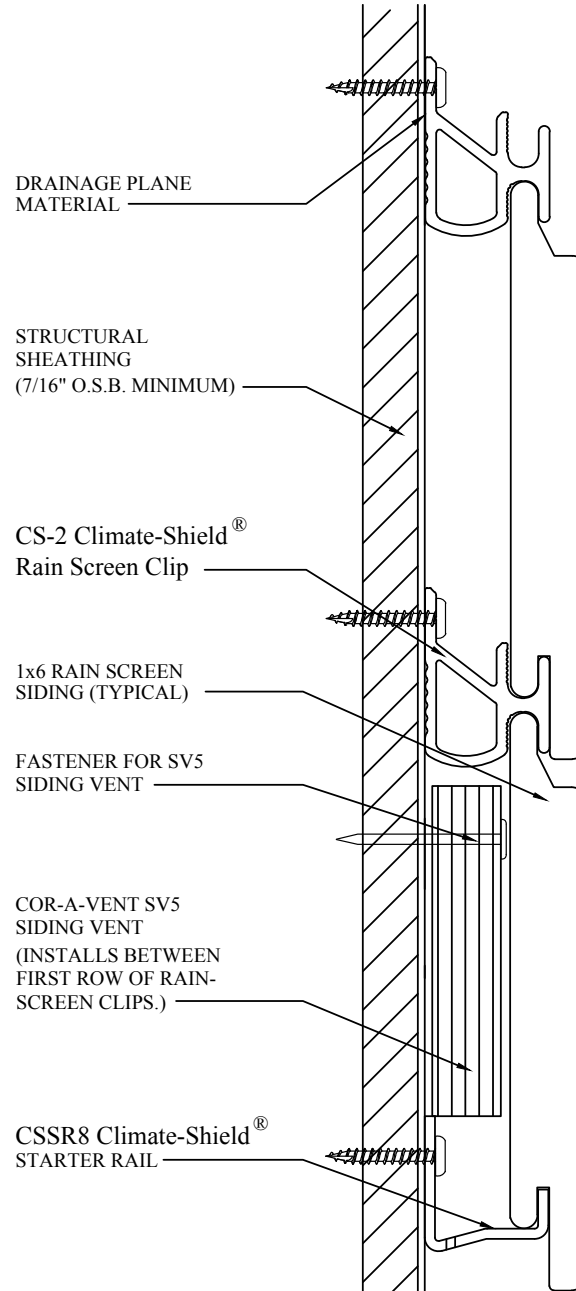
CROSS SECTION
